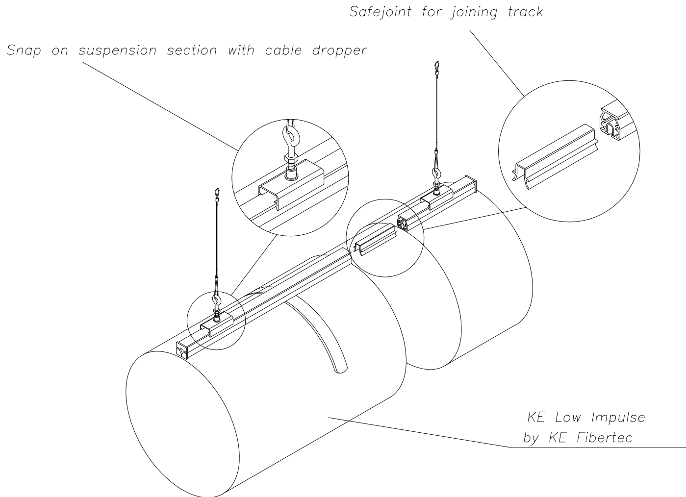
Safetrack Arch Suspension Detail for KE Fibertec Fabric Ducts (12 o'clock Attachment)
